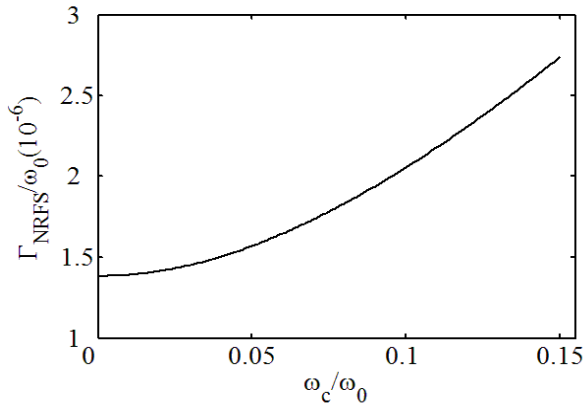
Fig. 2: The variation of normalized NRFS growth rate against the normalized cyclotron frequency
